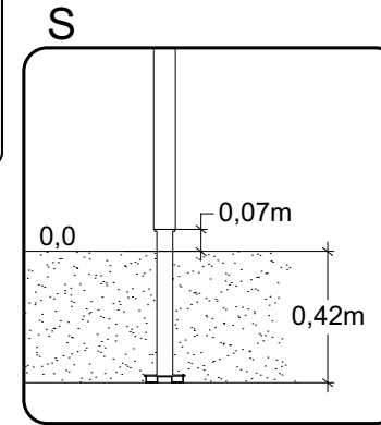
S Sunken Foundation 8113193
